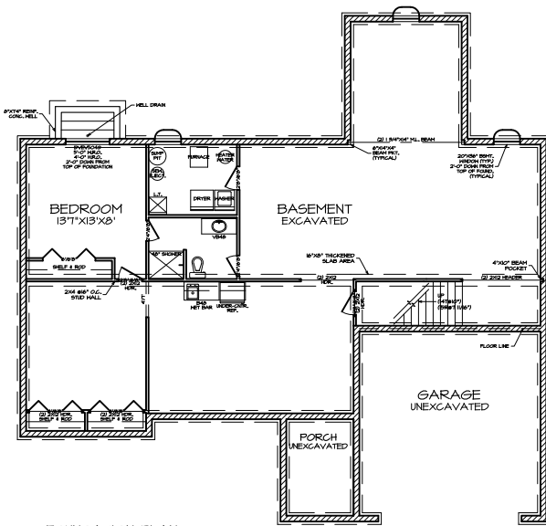
FOUNDATION PLAN A-2
