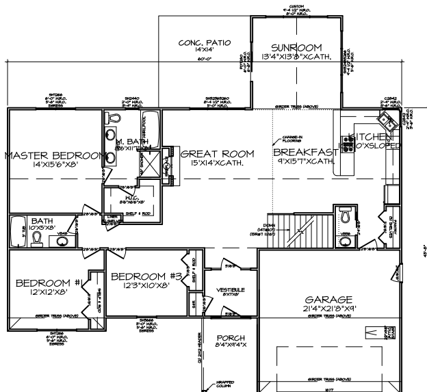
FIRST FLOOR PLAN A-3
